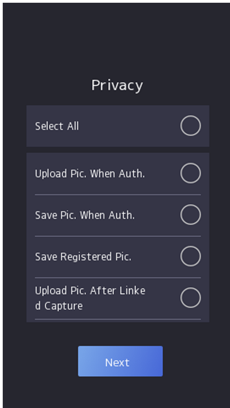
Figure 6-6 Privacy
