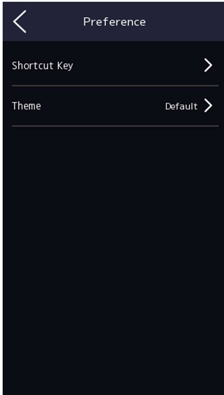
Figure 7-18 Preference Settings
