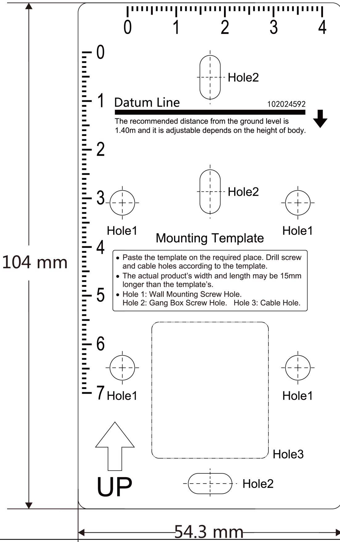
Figure 3-7 Mounting Template
