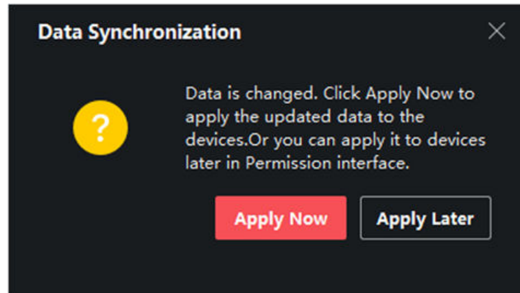
Figure 9-7 Data Synchronization
