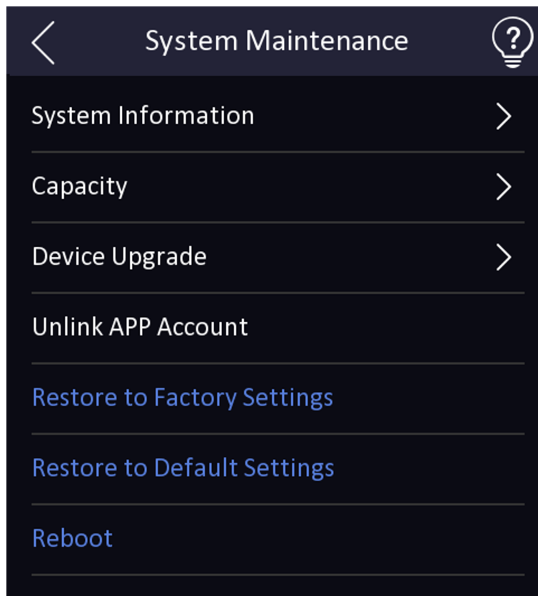
Figure 7-17 Maintenance Page
